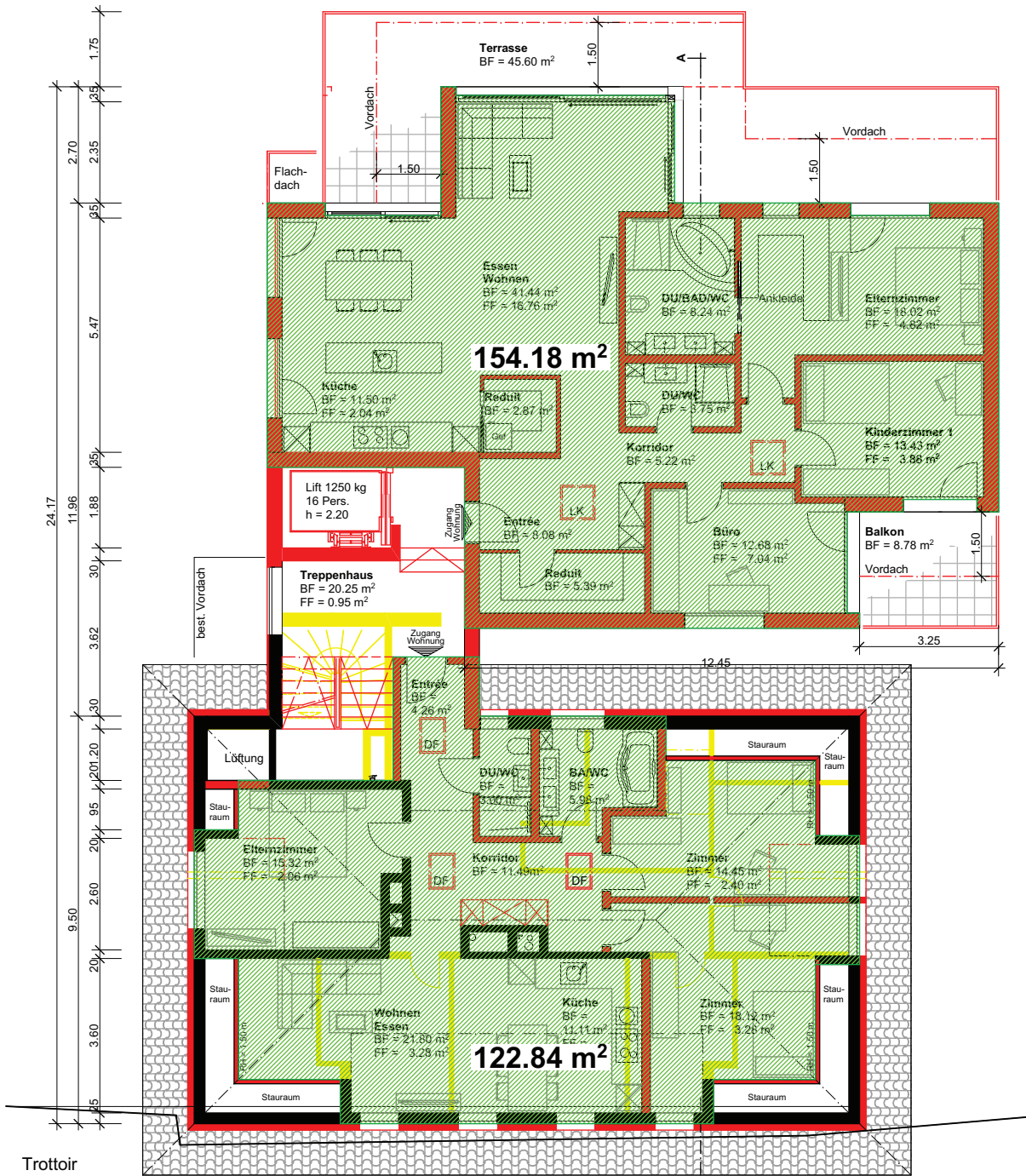
Grundriss Attika / DG Mst. 1:150 BGF = 154.18 m 2 + 122.84 m 2 = 277.02 m 2
